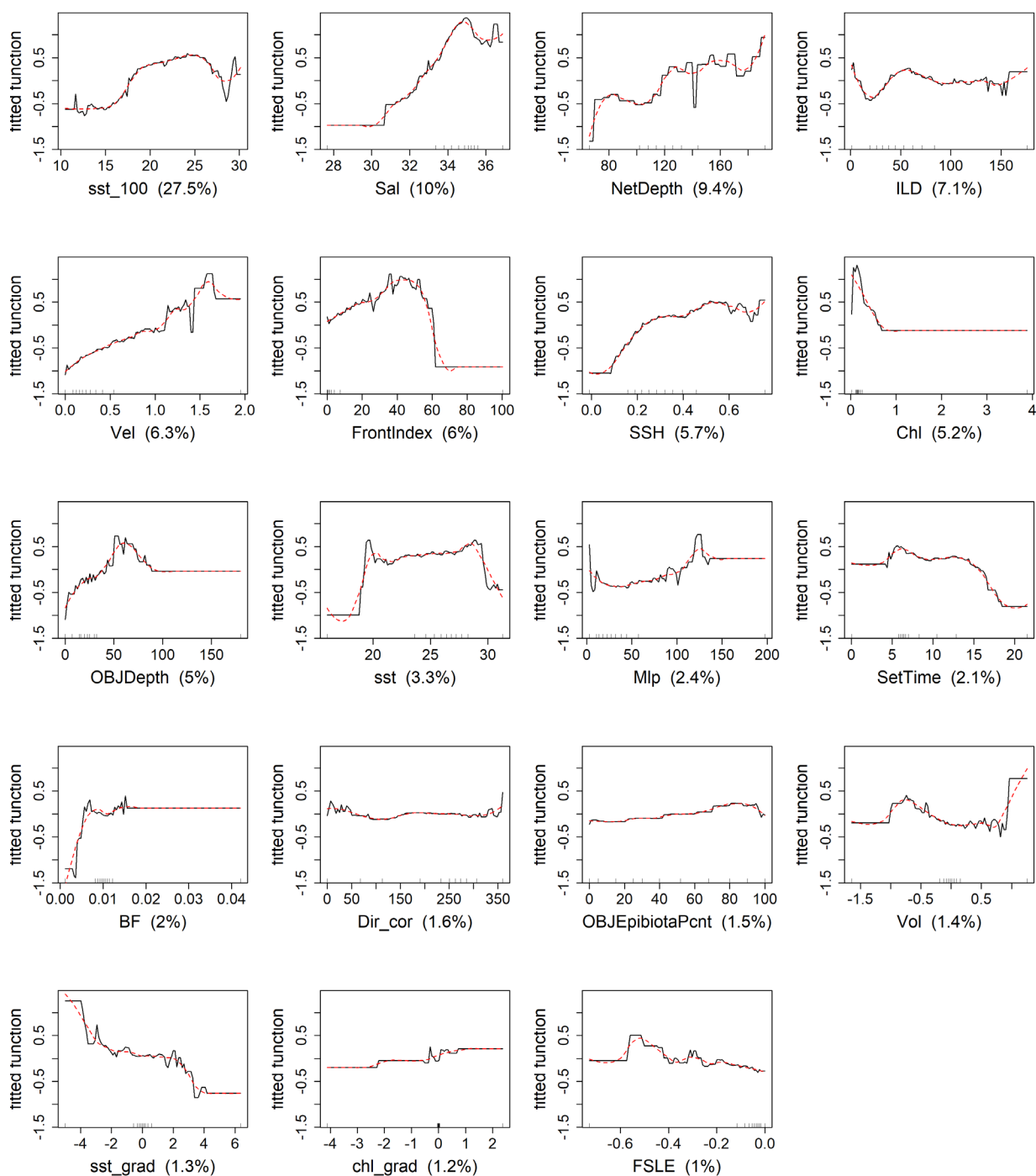
Figure 4. Partial dependence plots of presence–absence boosted regression trees (BRTs), showing relative probability of the presence of juvenile bigeye as a response to environmental and operational variables. Variable importance scores are listed for each variable in parenthesis.
